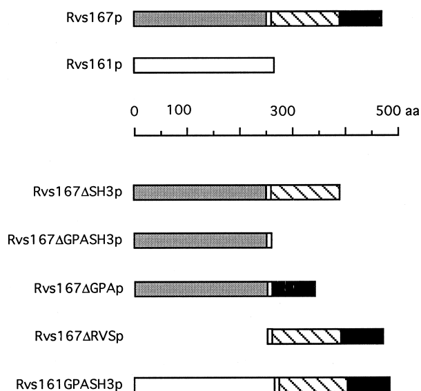
Fig. 1. Schematic representation of the different recombinant Rvs proteins. The wild-type Rvs161 and Rvs167 proteins are also shown. The domains of the proteins are represented as boxes (white box: RVS domain of Rvs161p; grey box: RVS domain of Rvs167p; hatched box: GPA domain; black box: SH3 domain).
